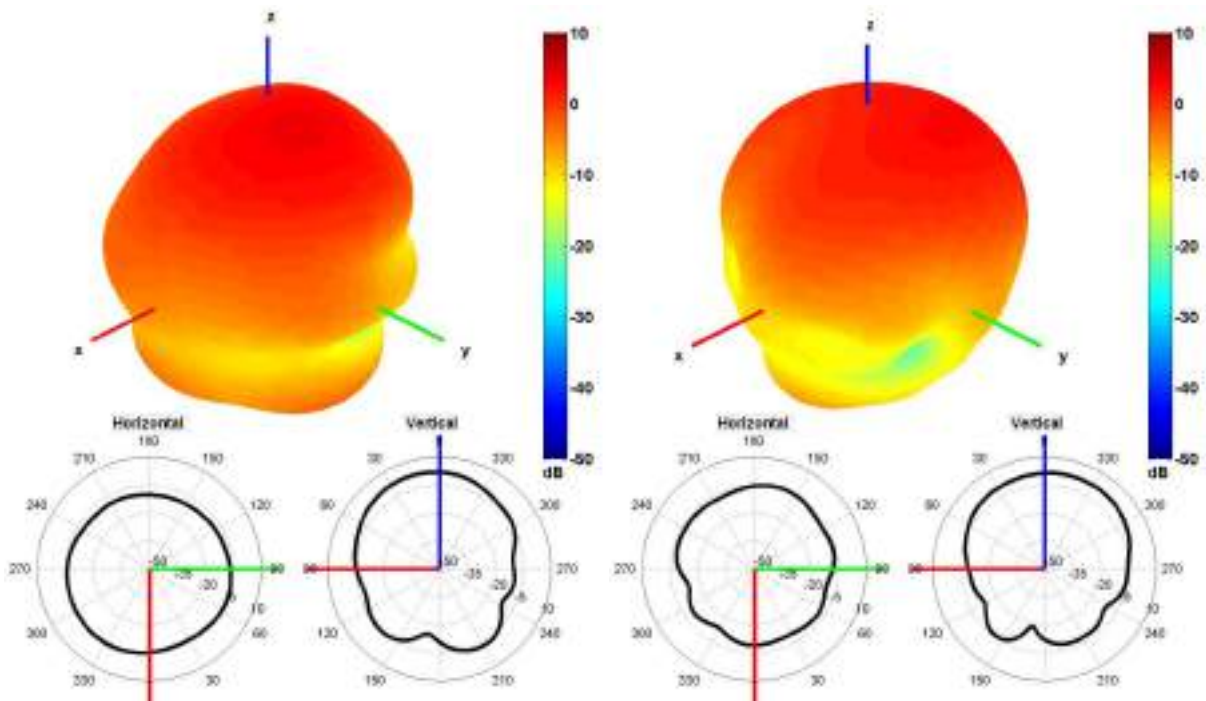
750 and 1176 MHz Radiation pattern
