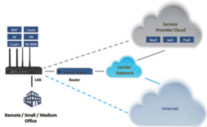
Figure 6 Branch Security and XaaS Gateway
