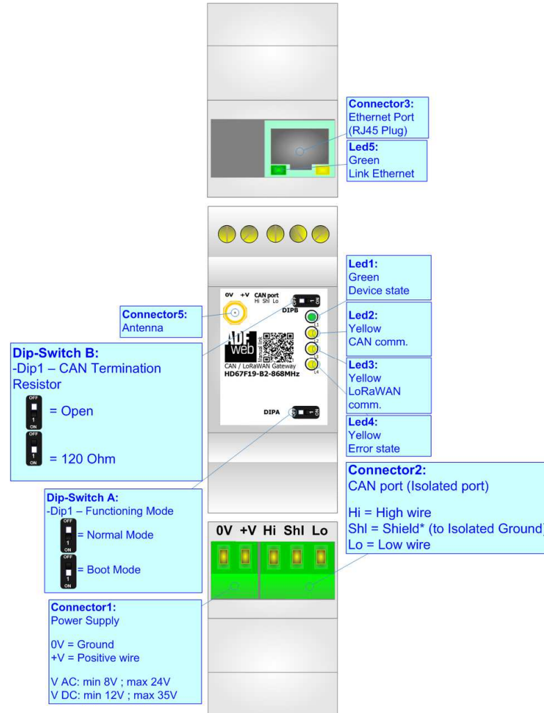
Figure 1: Connection scheme for HD67F19-B2-xxxMHz
