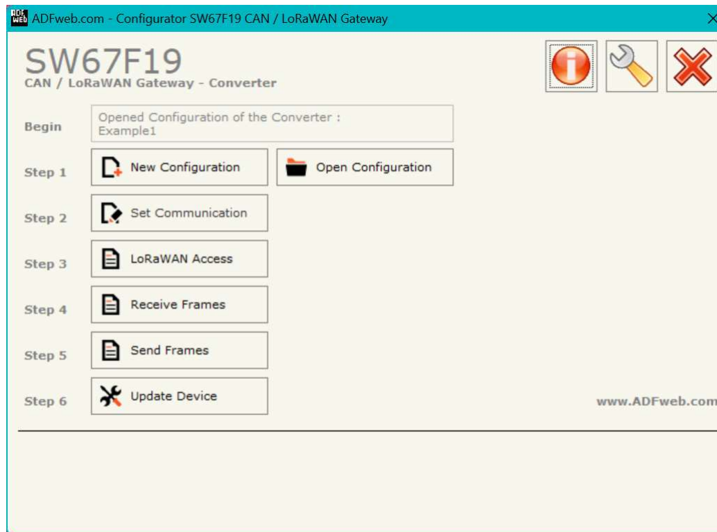
Figure 2: Main window for SW67F19
